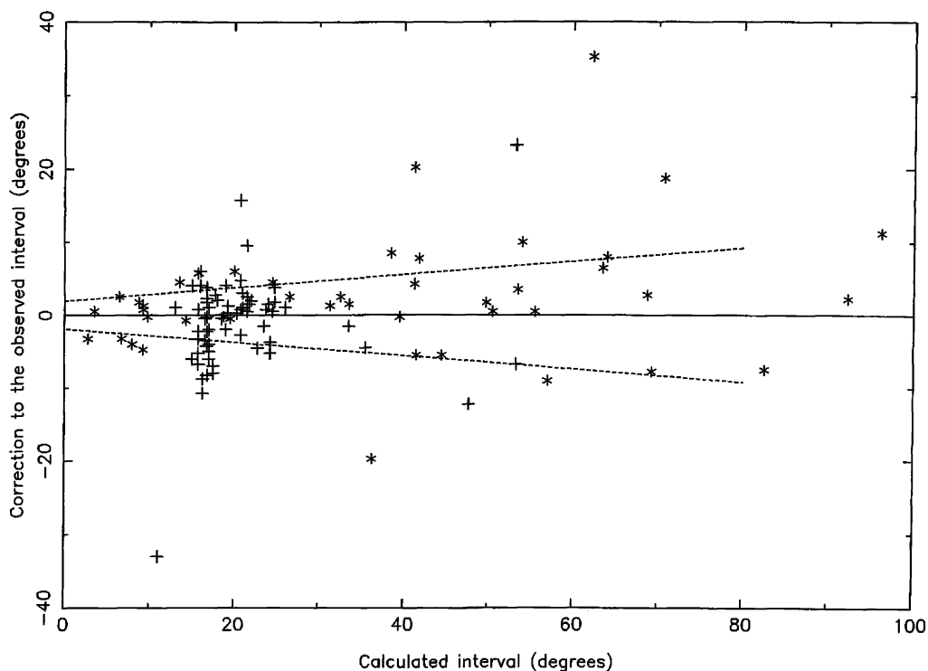
FIG. 2. The correction to the observed first contact interval and phase duration plotted against the calculated interval.
